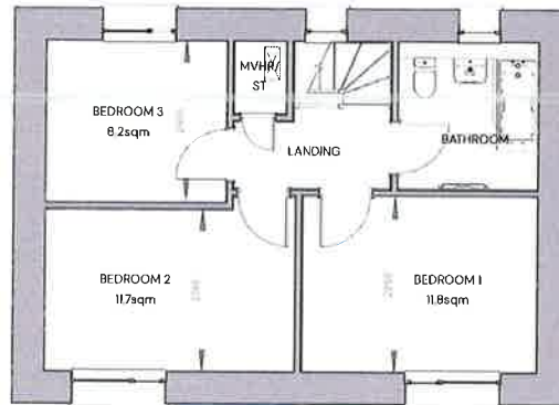
FIRST FLOORPLAN
