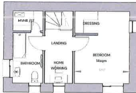
FIRST FLOORPLAN
